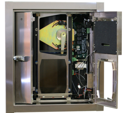
An inside look at the IRT-5000
