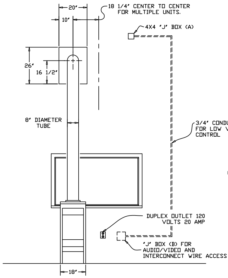
INTERIOR ELEVATION
