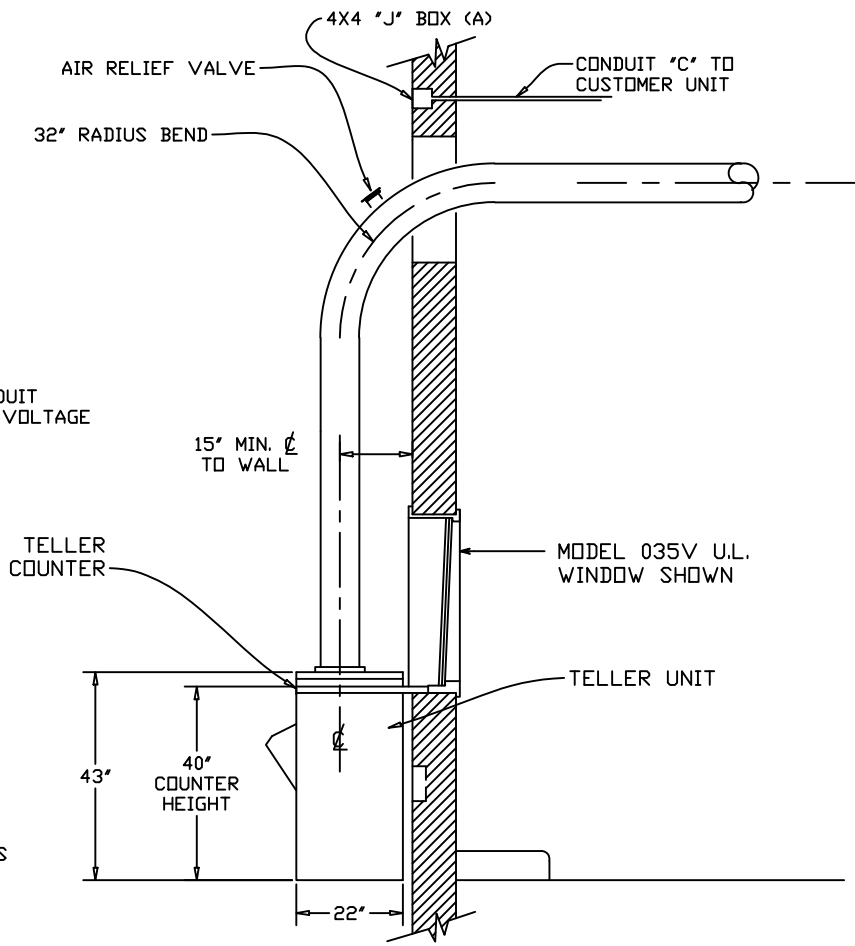
SECTION
