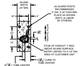
ISLAND DETAIL
