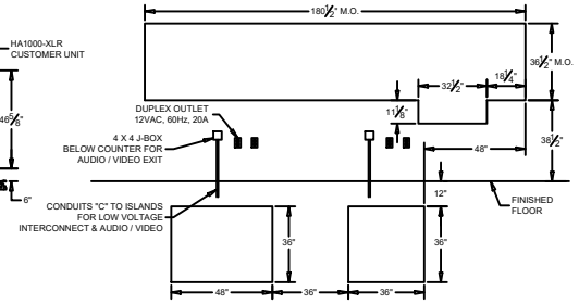
MASONRY DETAIL (FOR MODEL 315D U.L. WINDOW)
