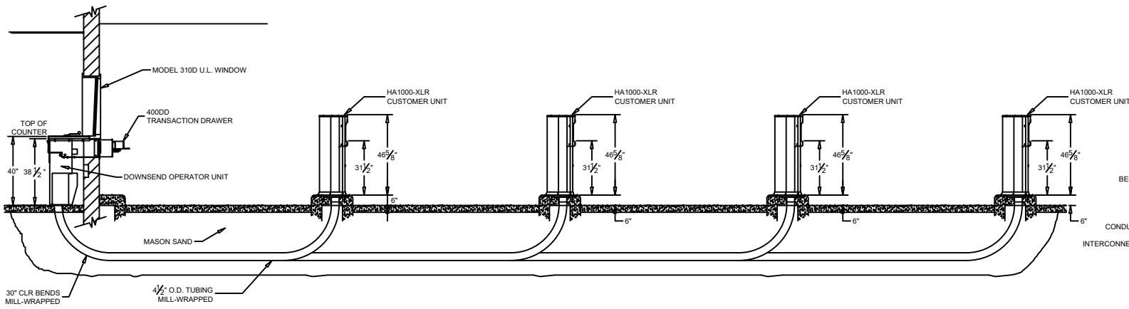
MINIMUM CANOPY HEIGHT OF 10'-0" SECTION
