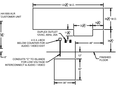
MASONRY DETAIL (FOR MODEL 310D U.L. WINDOW)
