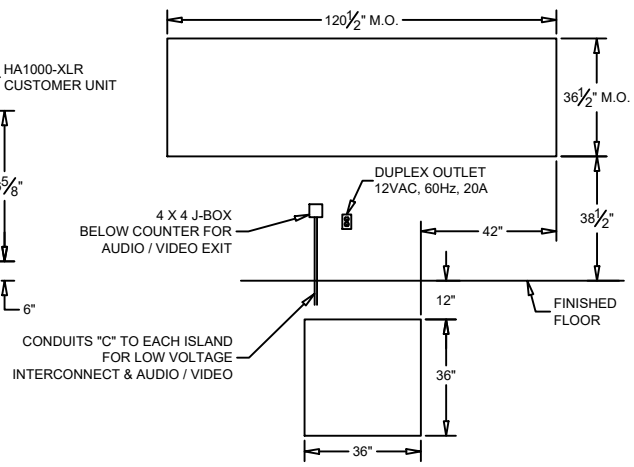
MASONRY DETAIL (FOR MODEL 310V U.L. WINDOW)
