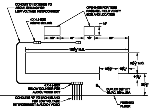
MASONRY DETAIL (FOR MODEL 318D U.L. WINDOW)
