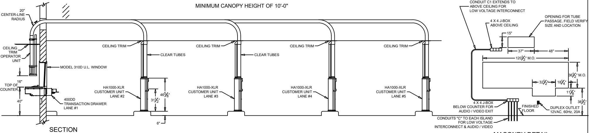
MASONRY DETAIL (FOR MODEL 310D U.L. WINDOW)
