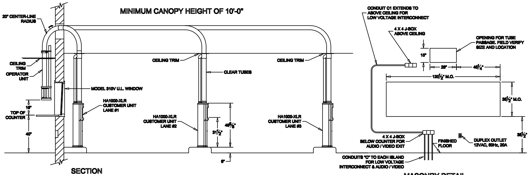
MASONRY DETAIL (FOR MODEL 310V U.L. WINDOW)
