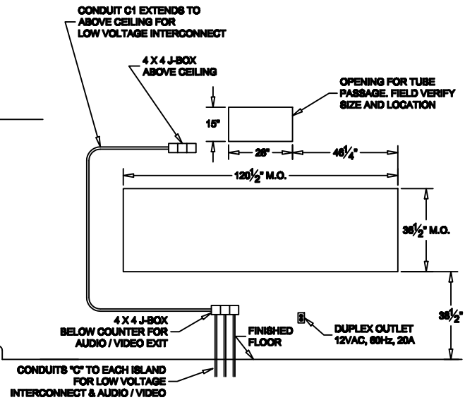
MASONRY DETAIL (FOR MODEL 310V U.L. WINDOW)
