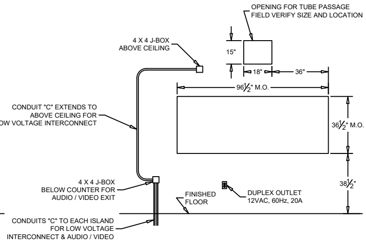
MASONRY DETAIL (FOR MODEL 038V U.L. WINDOW)
