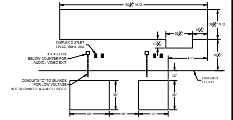
MASONRY DETAIL (FOR MODEL 315D U.L. WINDOW)
