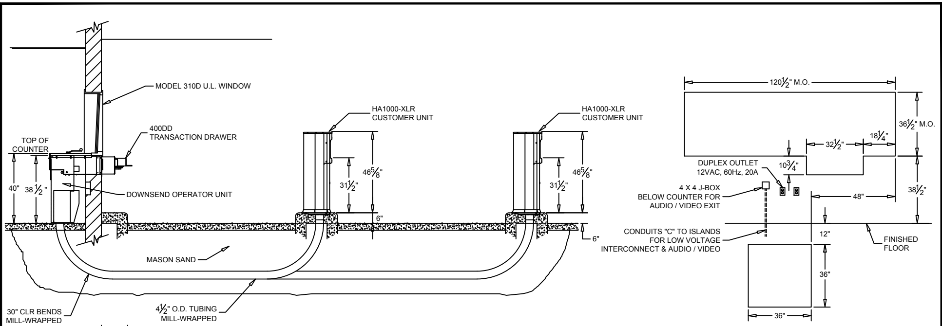
MASONRY DETAIL (FOR MODEL 310D U.L. WINDOW)
