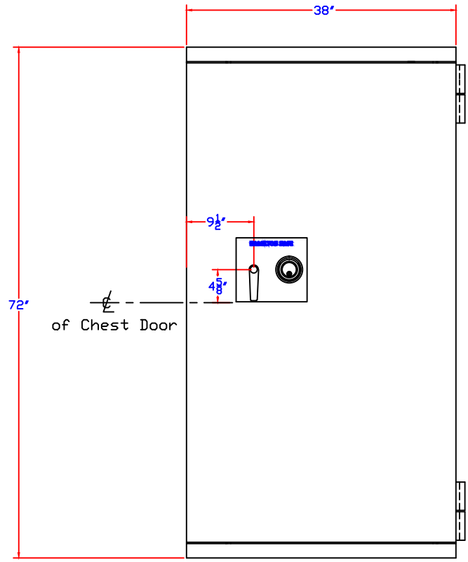
FRONT ELEVATION
