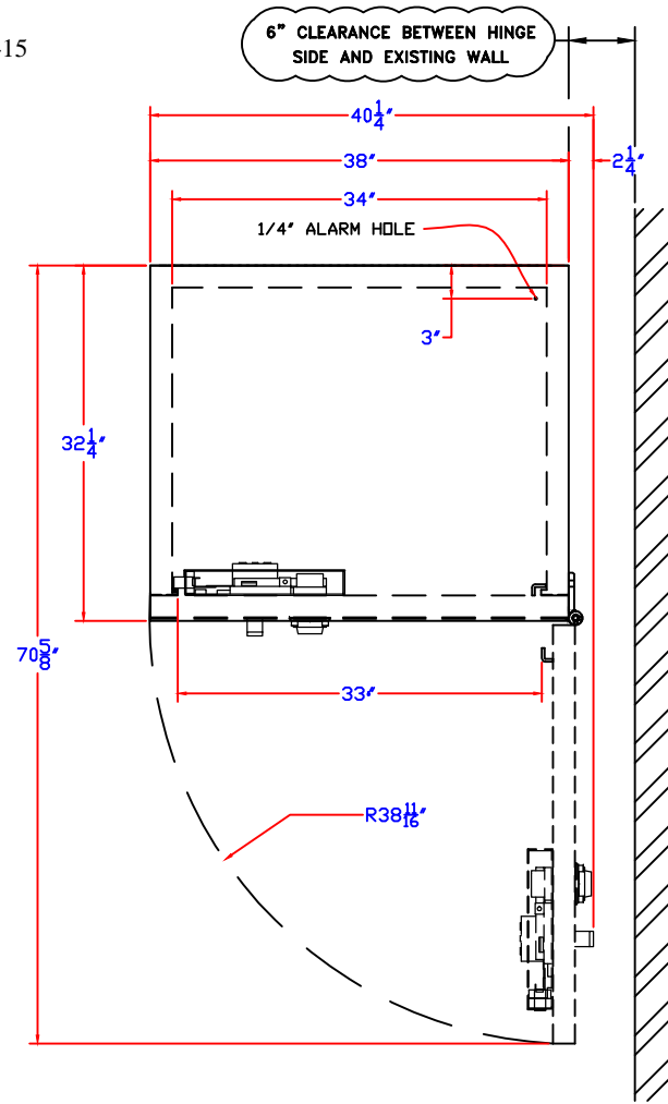
PLAN VIEW WITH DOOR OPEN AT 90°
