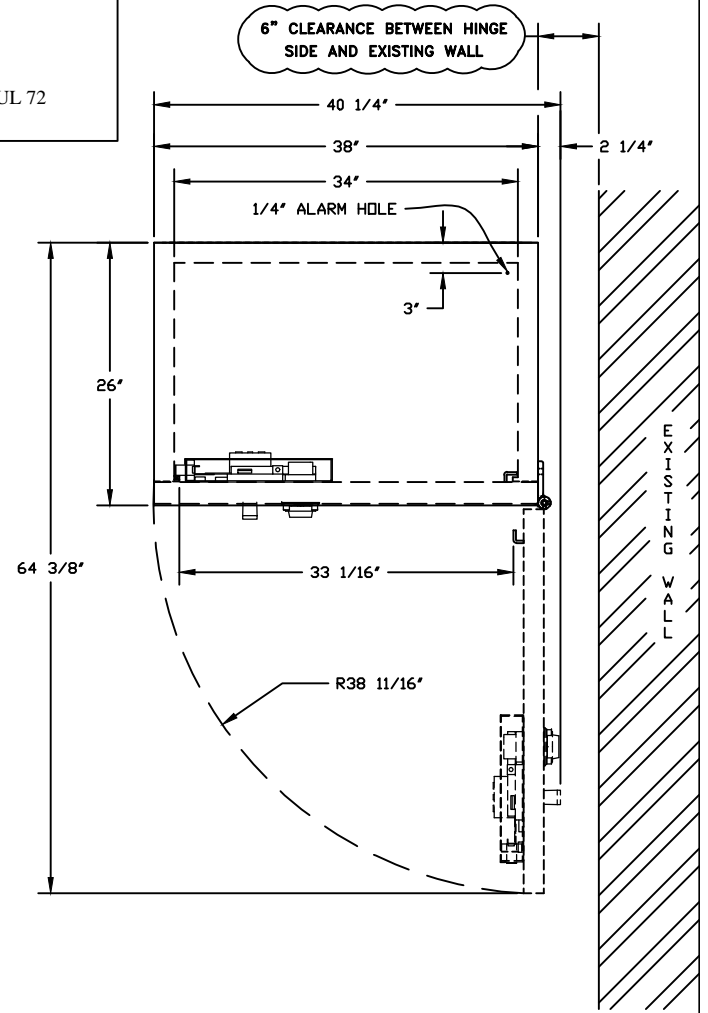
PLAN VIEW WITH DOOR OPEN AT 90°
