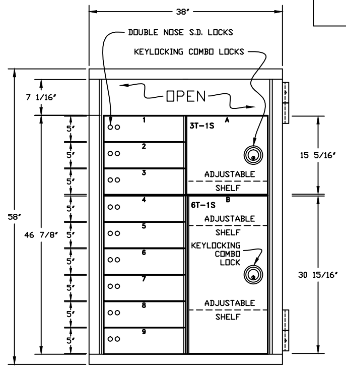
FRONT ELEVATION (DOOR REMOVED)
