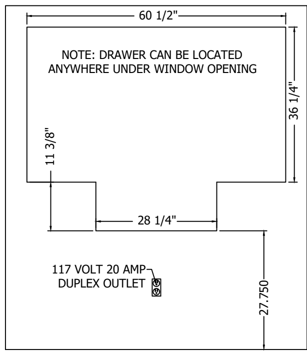
MASONRY OPENING INTERIOR
