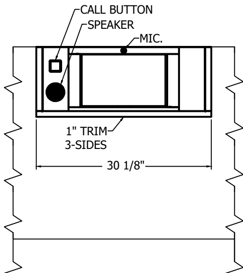
EXTERIOR ELEVATION
