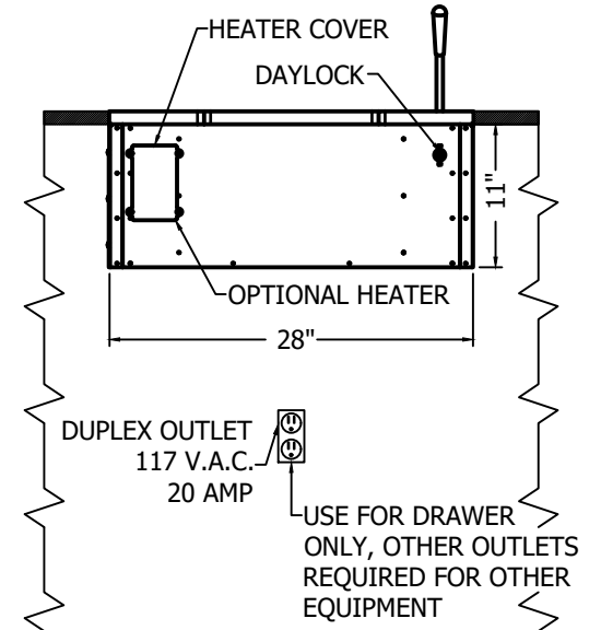
INTERIOR ELEVATION
