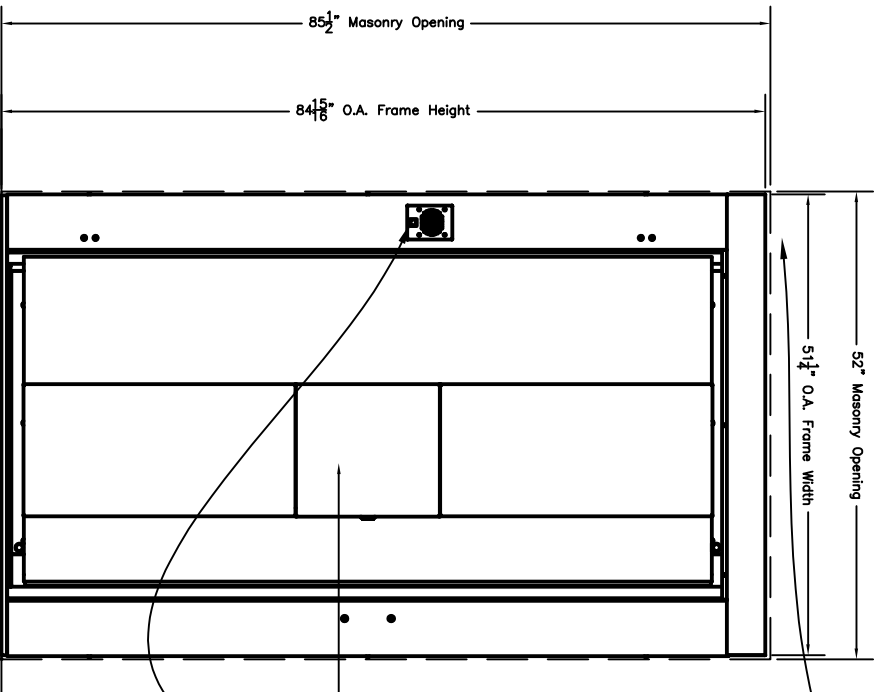
INTERIOR ELEVATION (SHOWN DAYGATE REMOVED)
