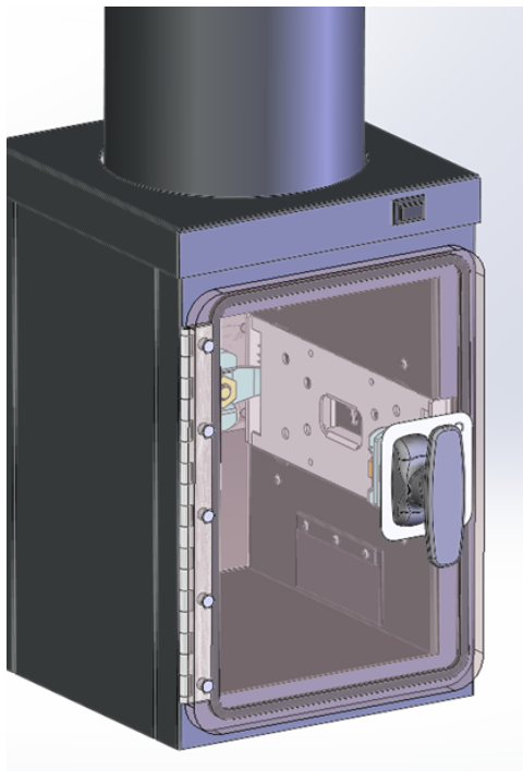
New T-handle latch design
