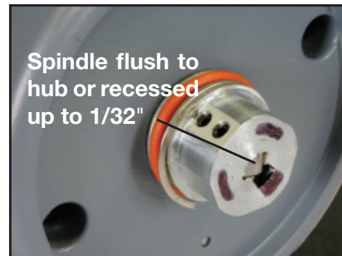
Figure 22 - Spindle Flush or Recessed
