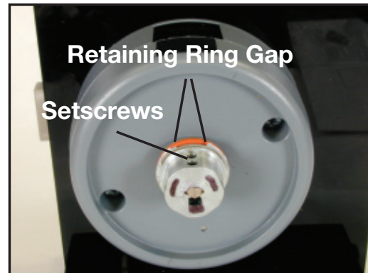
Figure 29 - Align Retaining Ring
