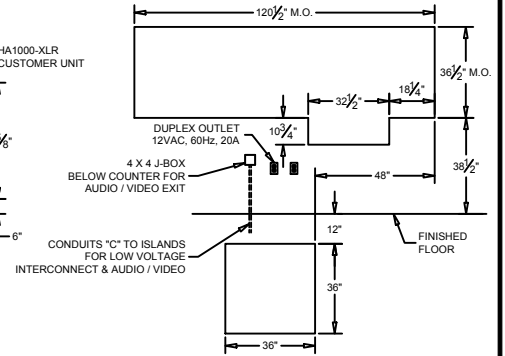
MASONRY DETAIL (FOR MODEL 310D U.L. WINDOW)
