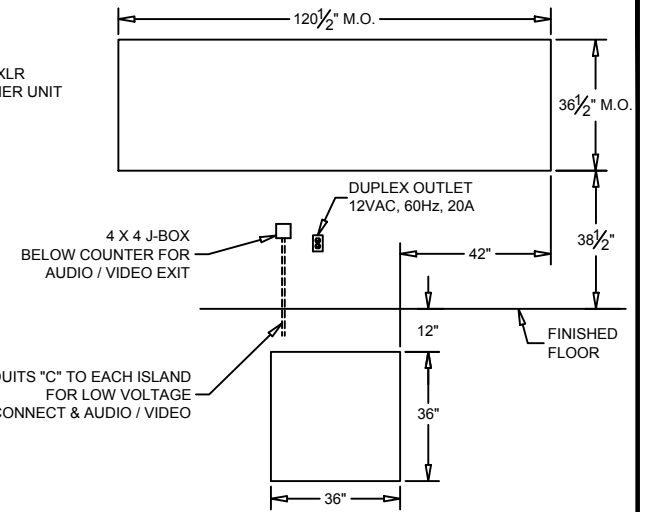
MASONRY DETAIL (FOR MODEL 310V U.L. WINDOW)
