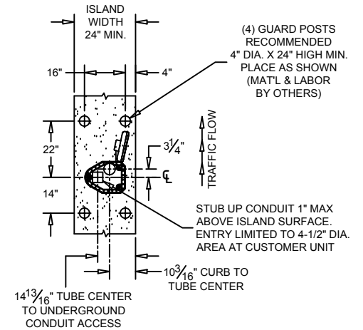
ISLAND DETAIL
